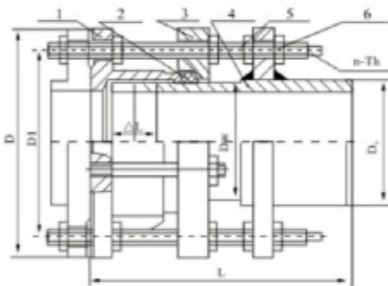
Single-flange structural drawing
