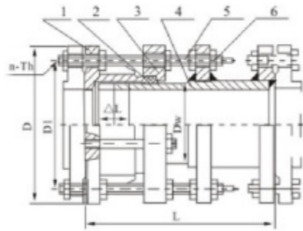
Detachable structural / dimensional drawing
