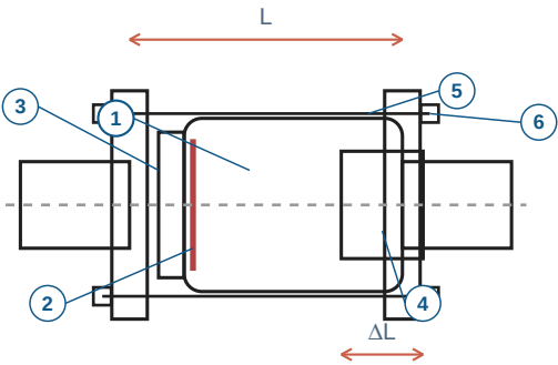
1 Body 3 Follower 5 Stud 2 Gasket 4 Limited short pipe 6 Nut Structural & adjustment drawing reference
