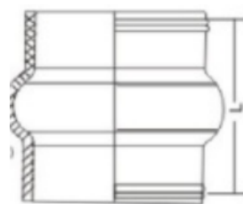
Clamp-end dimensional drawing
